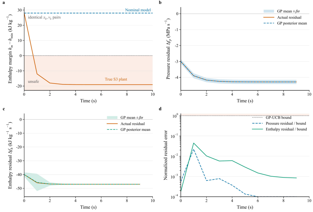
Figure 3. Direct model-mismatch diagnosis under the certificate-aligned S3 drift perturbation. (a) Nominal and true one-step enthalpy-margin responses from identical state-input pairs. (b,c) Pressure and enthalpy residual rates compared with the scenario-specific GP posterior mean and GP-UCB envelope ( \mu_{\text{GP}} \pm \beta\sigma_{\text{GP}} , \beta = 12.967 , N = 500 ). (d) Posterior residual error normalized by the GP-UCB bound; values below one lie inside the modeled envelope.
