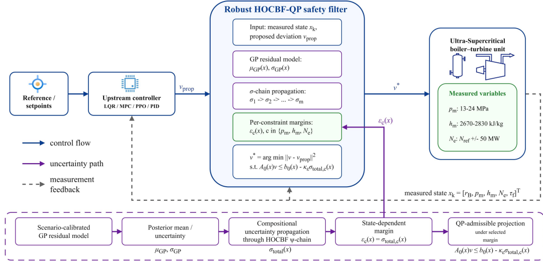
Figure 1. RoCBF-SF safety-filtering architecture. The upstream controller (LQR, MPC, PID, or learned policy) proposes a deviation command v_{prop} . The filter evaluates that command against current plant measurements and the GP residual model, then projects it to the nearest QP-admissible deviation command v^* under the selected margin through A(x)v \leq b(x) - \epsilon_c \sigma_{total}(x) . The physical actuator command is then reconstructed by Eq. (1).
