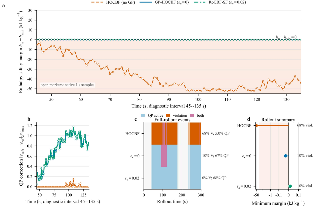
Figure 2. Closed-loop mechanism for representative seed 3 under the certificate-aligned S3 drift perturbation. (a,b) Enthalpy safety margin and normalized QP correction over the 45–135 s interval containing the onset and largest excursion. The shaded region marks violation of the lower enthalpy constraint. (c) Full 300 s event record. (d) Full-rollout minimum enthalpy margin and sample-level violation rate; the symmetric-log horizontal scale resolves the two near-zero margins while retaining the large no-GP excursion. Lines in (a,b) are interpolated on a 0.1 s display grid only for visual continuity; open markers are the native 1 s controller samples, and all statistics use native samples and the 10^{-2} counting tolerance defined in Eq. (12).
