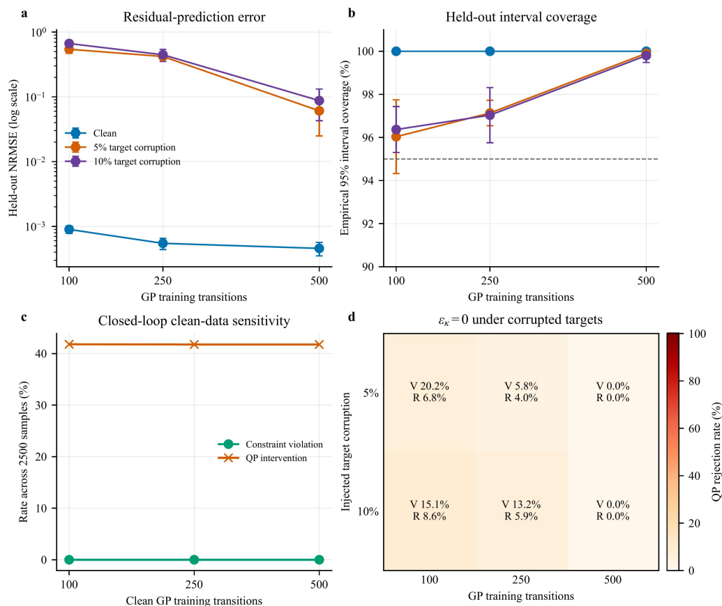
Figure 5. Controlled GP training-data sensitivity under S3. (a,b) Held-out residual NRMSE and empirical 95% interval coverage for 100, 250, and 500 selected transitions. Target corruption replaces a fixed training fraction with signed three-standard-deviation offsets. (c,d) Closed-loop violation and QP-rejection diagnostics under clean and corrupted training data. Each point aggregates five 500-sample rollouts. The 5% and 10% levels are synthetic fault-injection tests, not estimates of plant-data quality.
