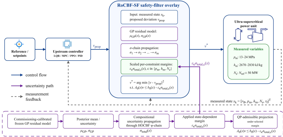
Figure 1. RoCBF-SF safety-filtering architecture. The upstream controller (LQR, MPC, PID, or learned policy) proposes a normalized deviation command v_{prop} . The filter evaluates that command against current plant measurements and the GP residual model, then projects it to the nearest QP-admissible deviation command v^* under A(x)v \leq b(x) - \epsilon_k \sigma_{total}(x) . The physical command is reconstructed with S_u by Eq. (1).
