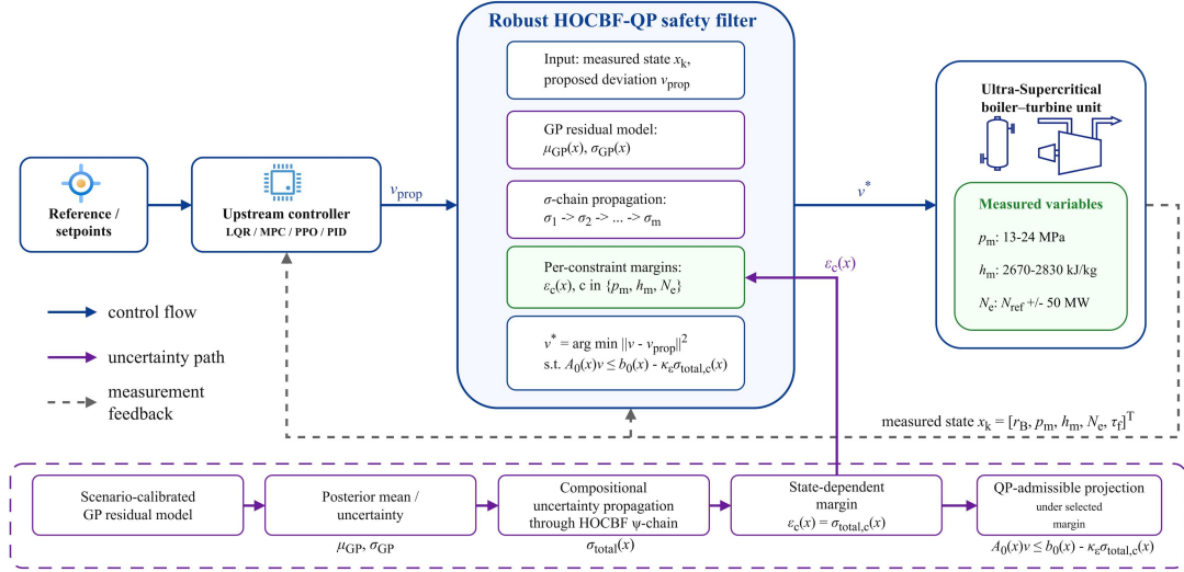
Figure 1. RoCBF-SF safety-filtering architecture. The upstream controller (LQR, MPC, PID, or learned policy) proposes a deviation command v_{\text{prop}} . The filter evaluates that command against current plant measurements and the GP residual model, then projects it to the nearest QP-admissible deviation command v^* under the selected margin through A(x)v \leq b(x) - \epsilon_k \sigma_{\text{total}}(x) . The physical actuator command is then reconstructed by Eq. (1).
