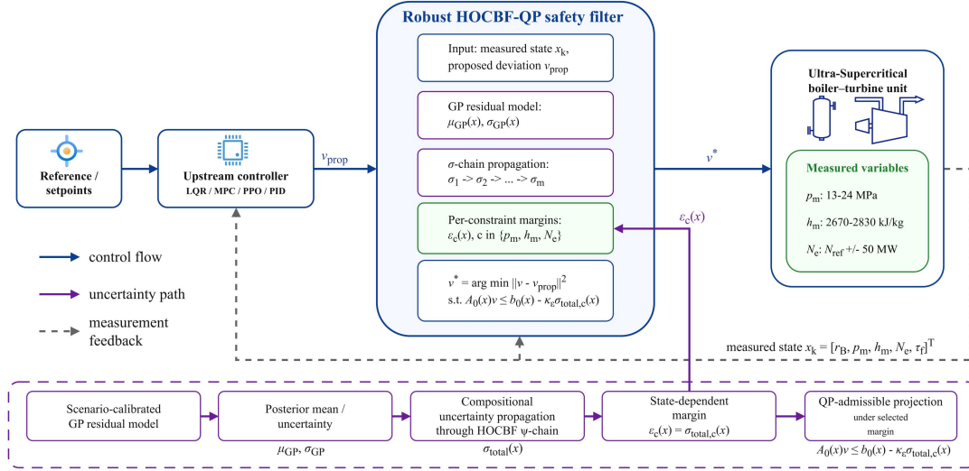
Figure 1. RoCBF-SF safety-filtering architecture. The upstream controller (LQR, MPC, PID, or learned policy) proposes a deviation command v_{\text{prop}} . The filter evaluates that command against current plant measurements and the GP residual model, then projects it to the nearest QP-admissible deviation command v^* under the selected margin through A(x)v \leq b(x) - \epsilon_{\kappa}\sigma_{\text{total}}(x) . The physical actuator command is then reconstructed by Eq. (1).
