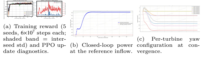
Figure 4: 3×3 grid farm closed-loop behavior. Reference inflow for (b,c) is (\phi, v) = (270^\circ, 11.4 \text{ m/s}) .
