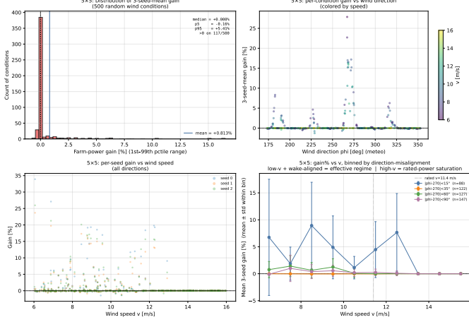
Figure 6: 5x5 distribution-wise evaluation under the optimized configuration. Aligned-cube gain is +4.70% ( n=51 , 3-seed mean), transferring 95.7% of the 3x3 headline (+4.91%). The regime decomposition reproduces the same two-tier structure observed at 3x3: gains are concentrated in the aligned-cube envelope and near-zero elsewhere. The earlier +0.98% result was an artifact of missing turbine position encoding (USE_POSITIONS flag disabled).
