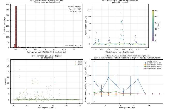
Figure 6: 5×5 distribution-wise evaluation under the optimized configuration. Aligned-cube gain is +4.70% ( n=51 , 3-seed mean), transferring 95.7% of the 3×3 headline (+4.91%). The regime decomposition reproduces the same two-tier structure observed at 3×3: gains are concentrated in the aligned-cube envelope and near-zero elsewhere. The earlier +0.98% result was an artifact of missing turbine position encoding (USE_POSITIONS flag disabled).
