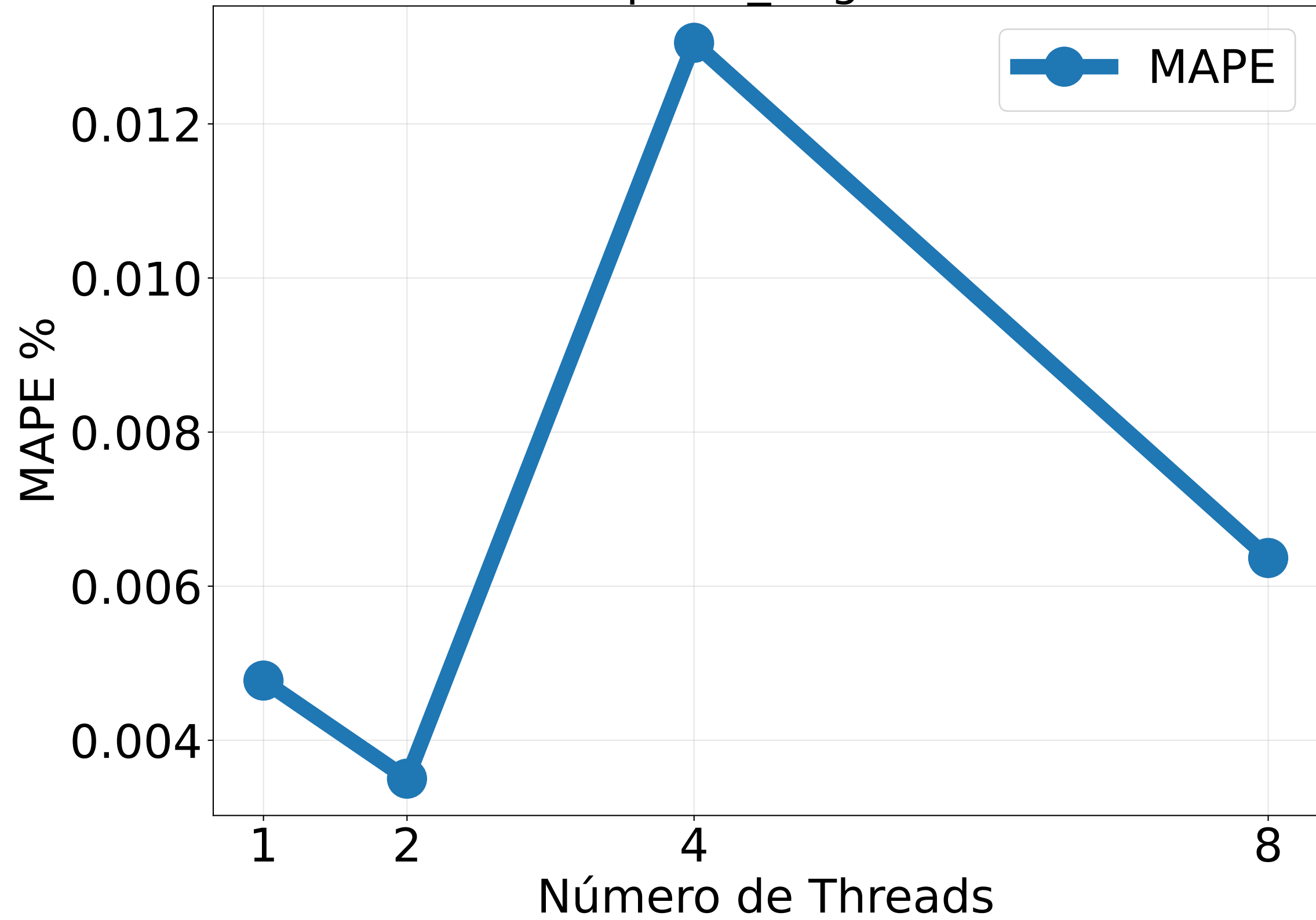
PI perfo_large 20
