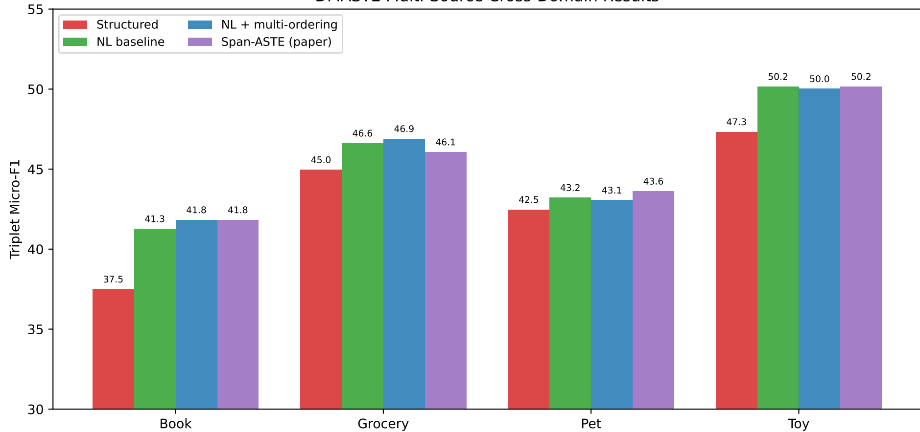
DMASTE Multi-Source Cross-Domain Results
