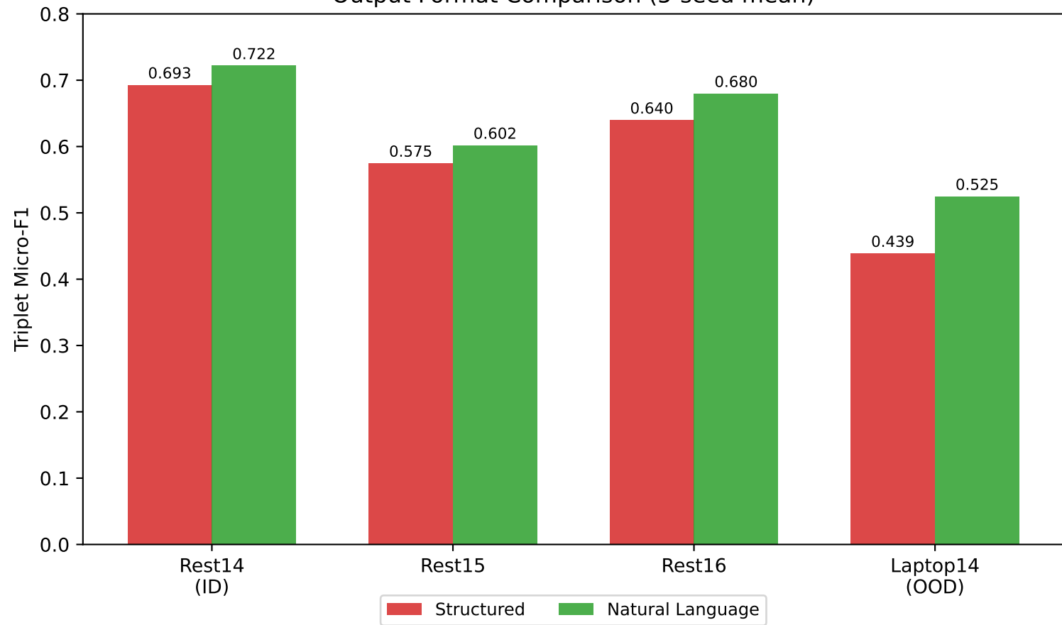
Output Format Comparison (5-seed mean)
