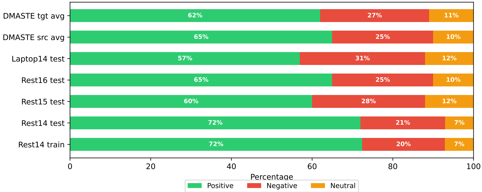
Polarity Distribution by Dataset
