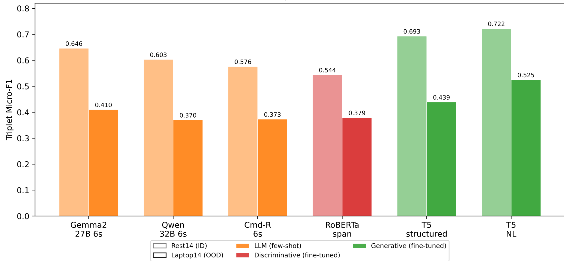
Cross-Method Comparison on SemEval ASTE
