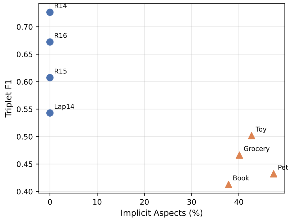
Dataset Characteristics vs. Model Performance
