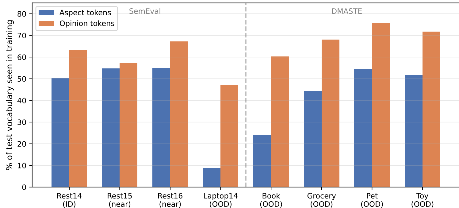
Vocabulary Overlap Between Training and Test Sets
