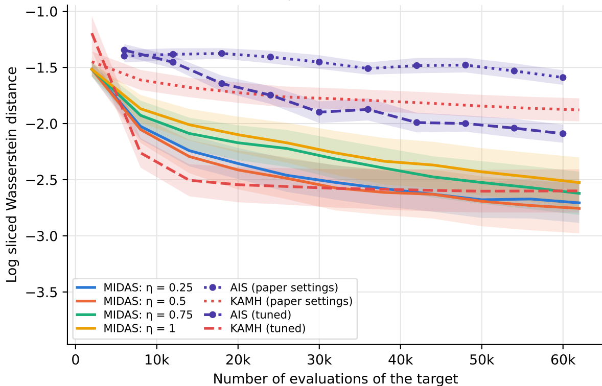
Anisotropic Gaussian mixture
