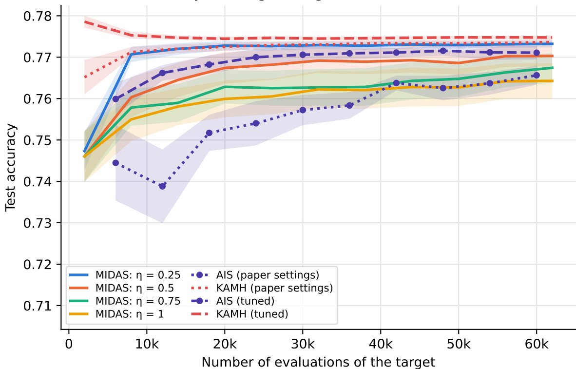
Bayesian logistic regression (waveform)
