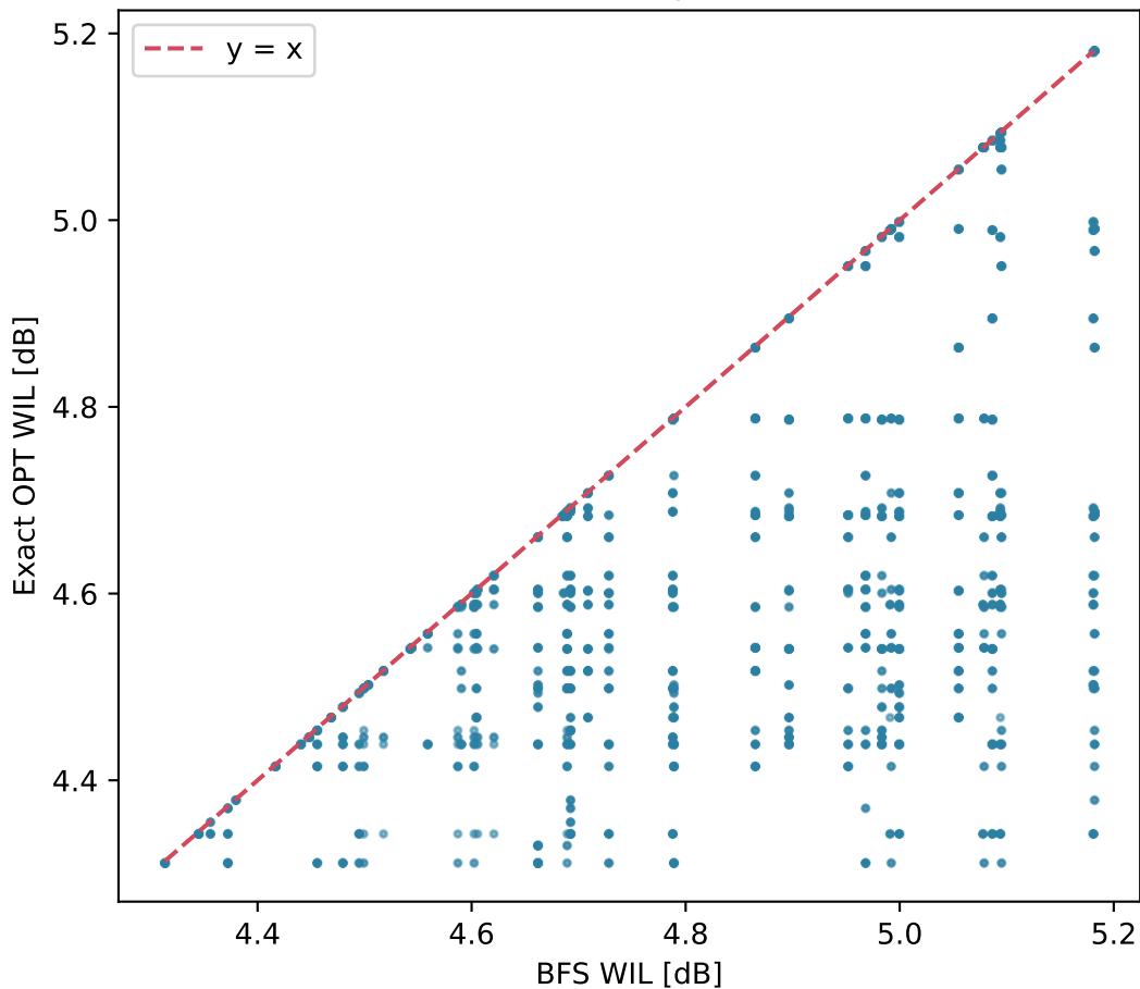
BFS versus optimum
