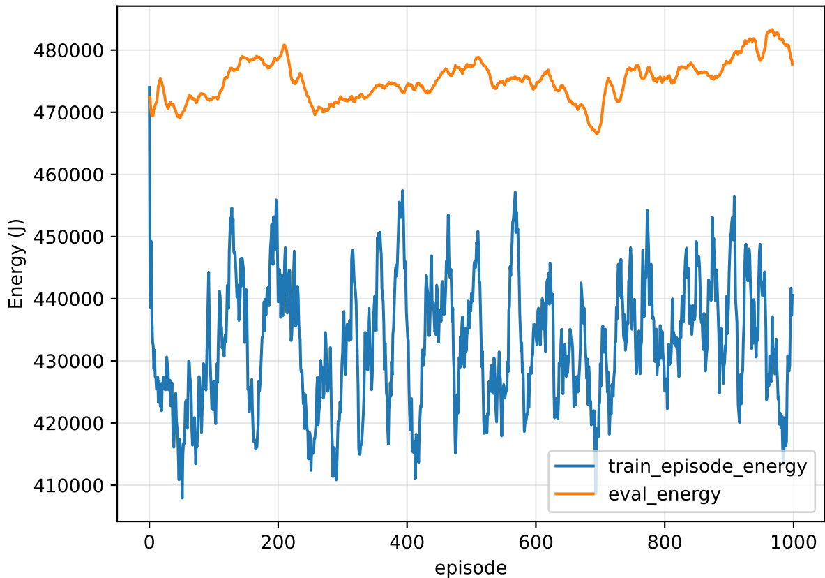
PD3QN Convergence: Energy
