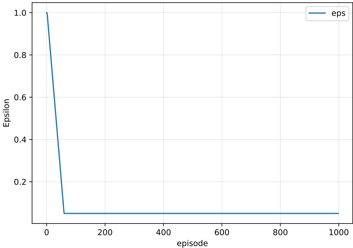
PD3QN: Epsilon Schedule
