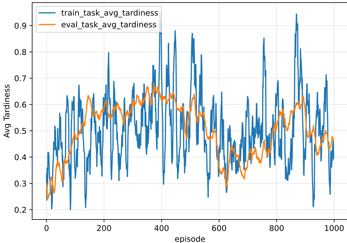
PD3QN Convergence: Task Avg Tardiness
