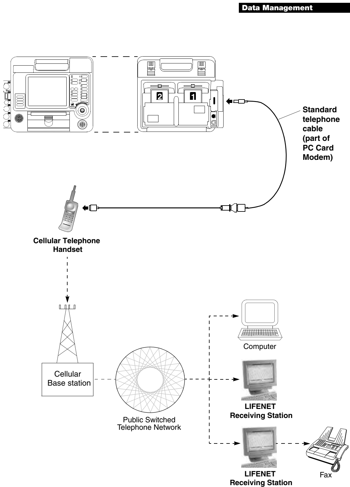
Figure 6-3 Equipment Connections for Internal Modem – Analog Cellular
