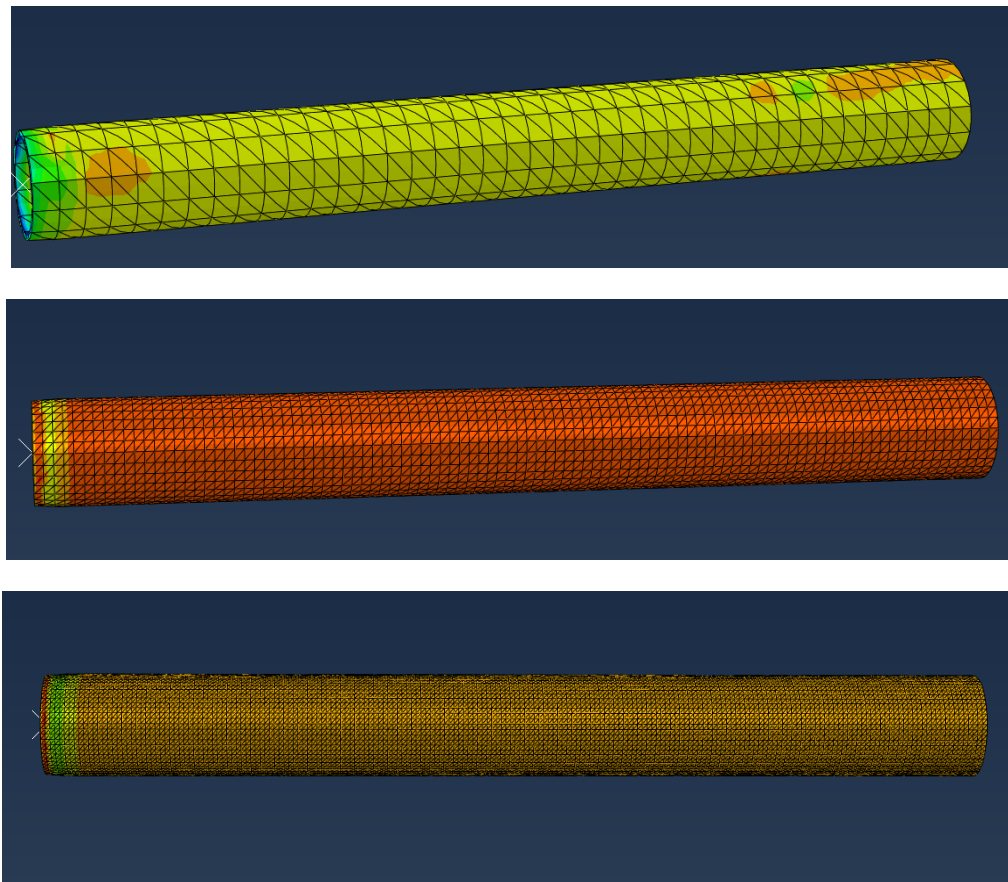
Figure: cylinder in compression in Abaqus
