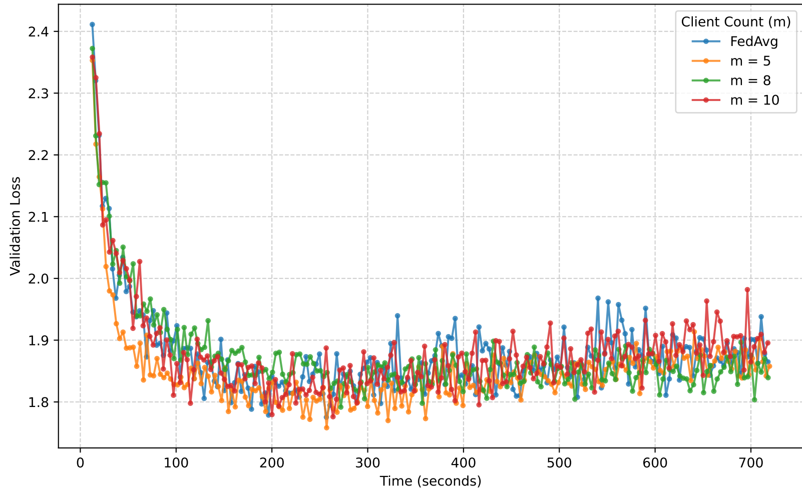
Federated Learning Analysis: cifar10 (fs=0.0)
