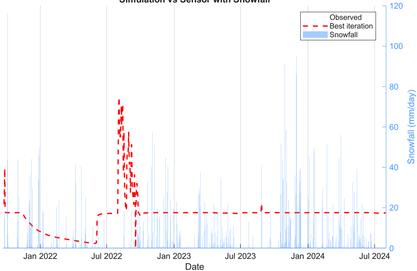
Simulation vs Sensor with Snowfall
