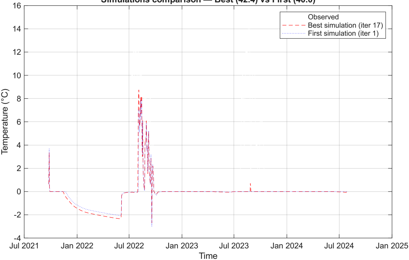
Simulations comparison — Best (42.4) vs First (40.0)
