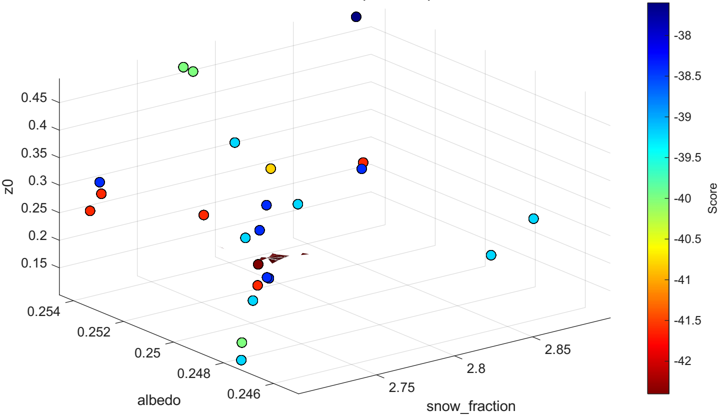
Isosurface forcée ( \geq -41.60 )
