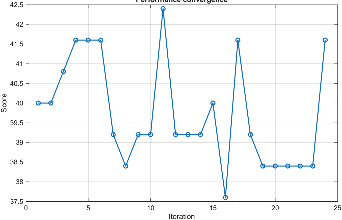
Performance convergence
