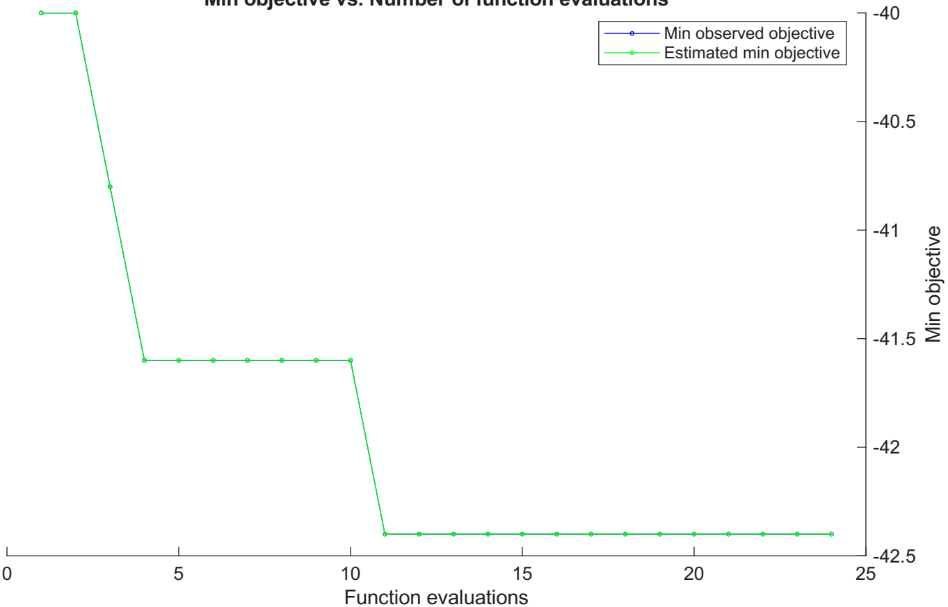
Min objective vs. Number of function evaluations
