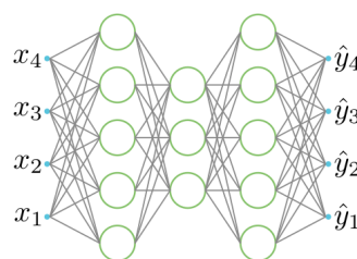
(c) Encoder-Decoder.
