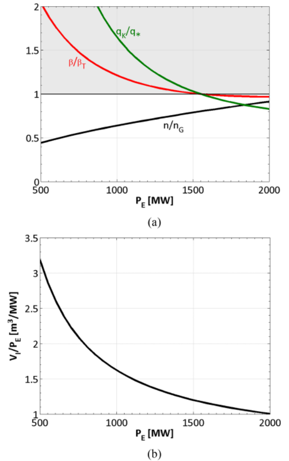
FIG. 8. (a) Curves of \bar{n}/n_G , \beta/\beta_T , and q_k/q_* as a function of P_E for H = 1 , B_{\max} = 13 \text{ T} assuming that f_B/f_{NC} = 1 . Successful operation corresponds to the unshaded region. (b) Corresponding curve of V_I/P_E versus P_E .
