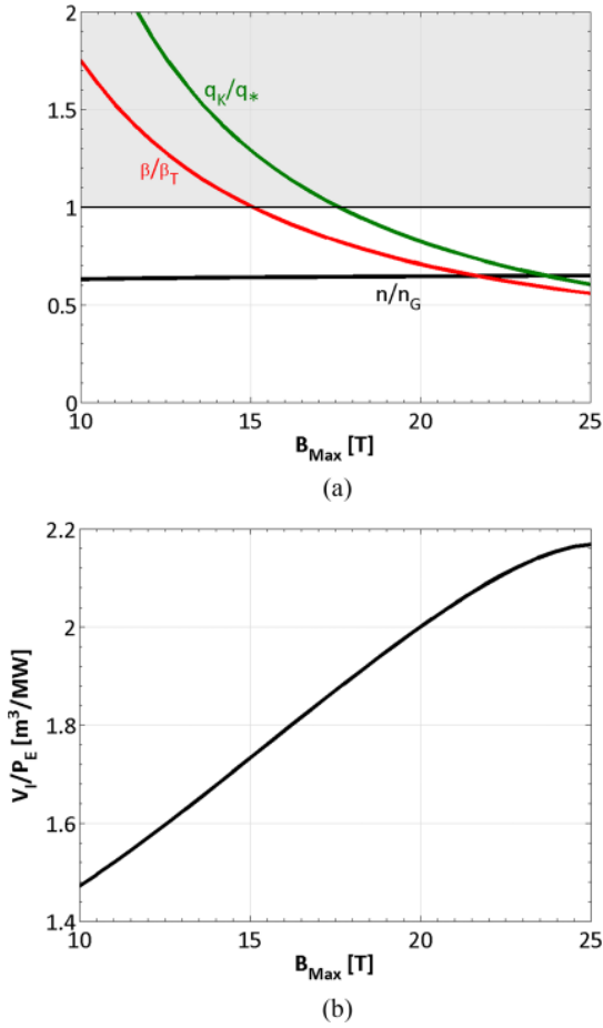
FIG. 7. (a) Curves of \bar{n}/n_G , \beta/\beta_T , and q_k/q_* as a function of B_{\max} for H = 1 assuming that f_B/f_{NC} = 1 . Successful operation corresponds to the unshaded region. (b) Corresponding curve of V_I/P_E versus B_{\max} .
