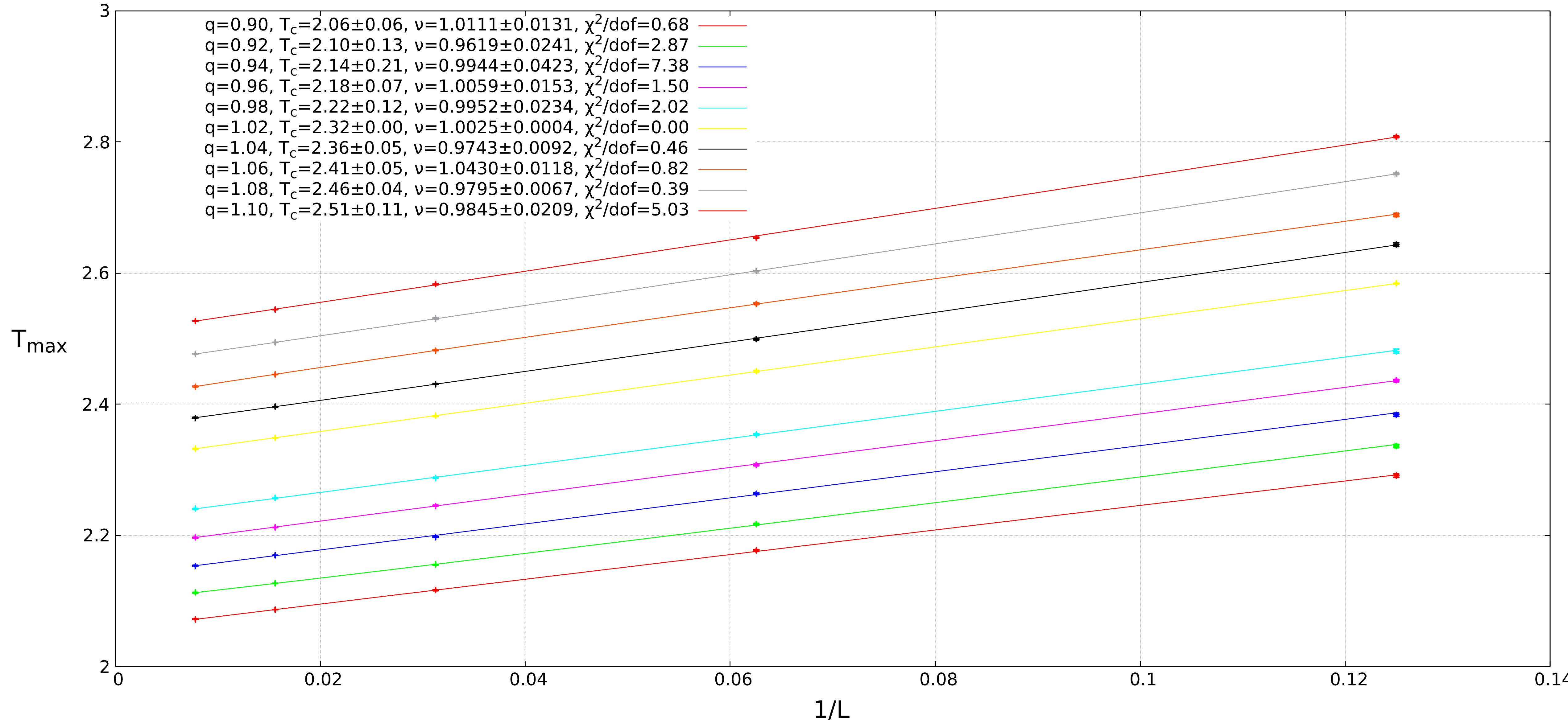
Peak location of \chi_m
