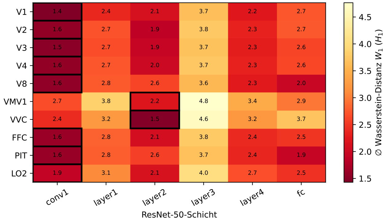
Topologische Distanz H_1 — ResNet-50 vs. Glasser-Areale (Ø S1-S3)
