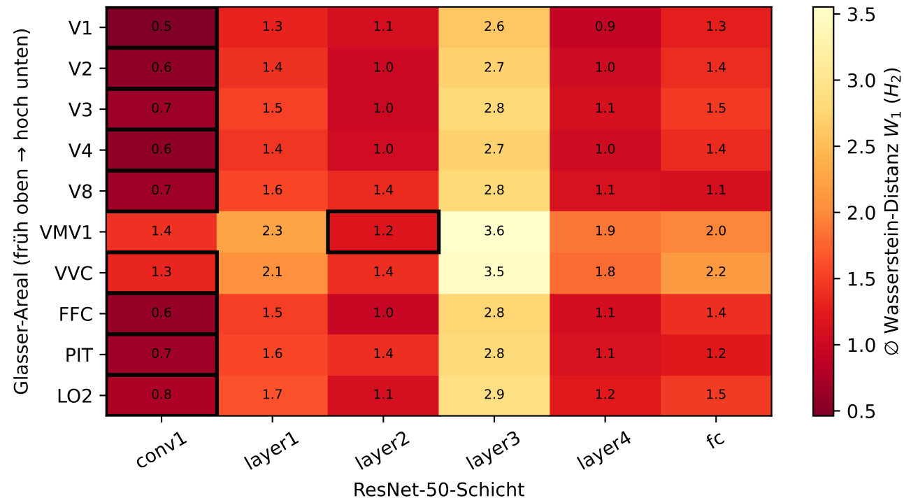
Topologische Distanz H_2 — ResNet-50 vs. Glasser-Areale (Ø S1-S3)
