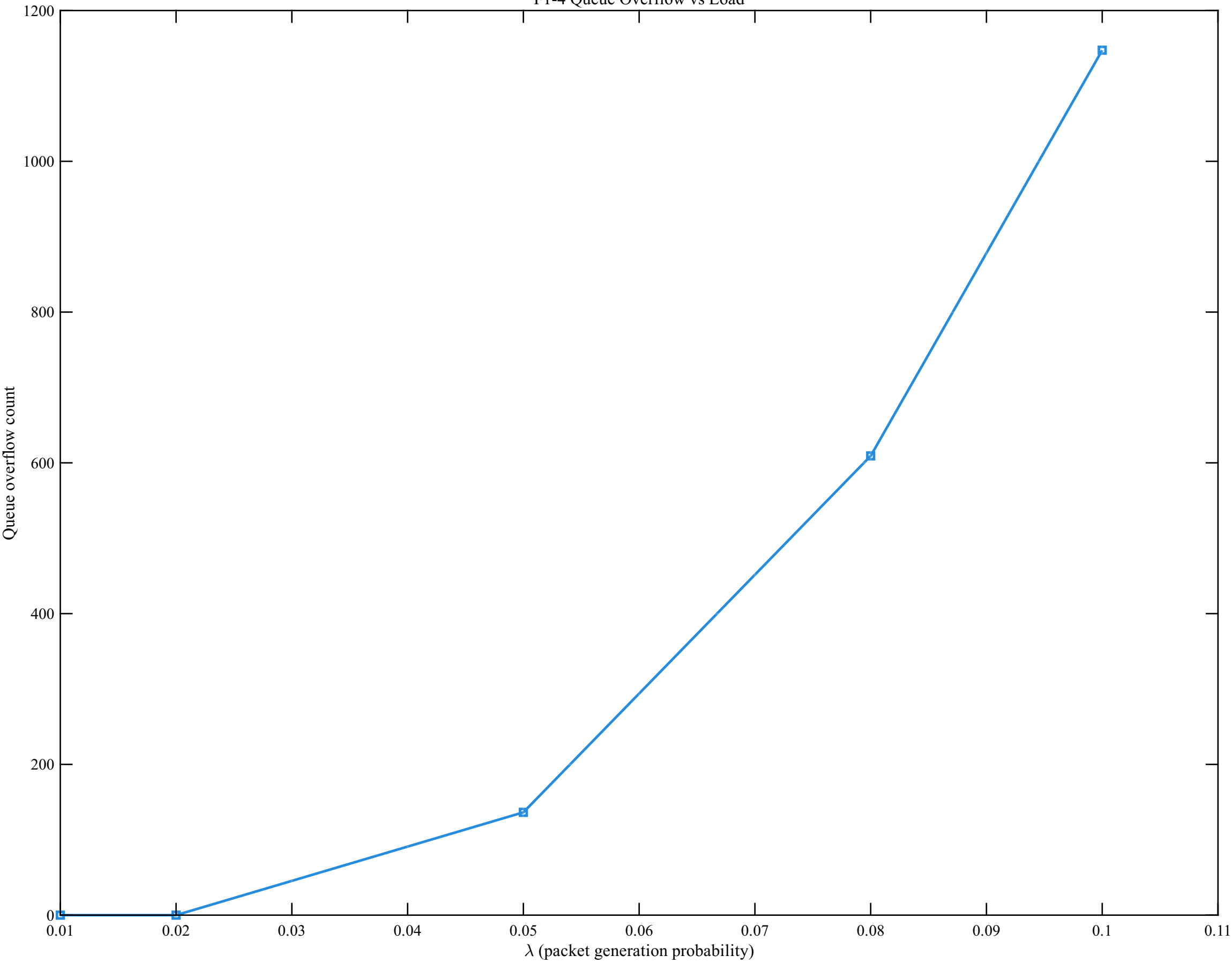
F1-4 Queue Overflow vs Load
