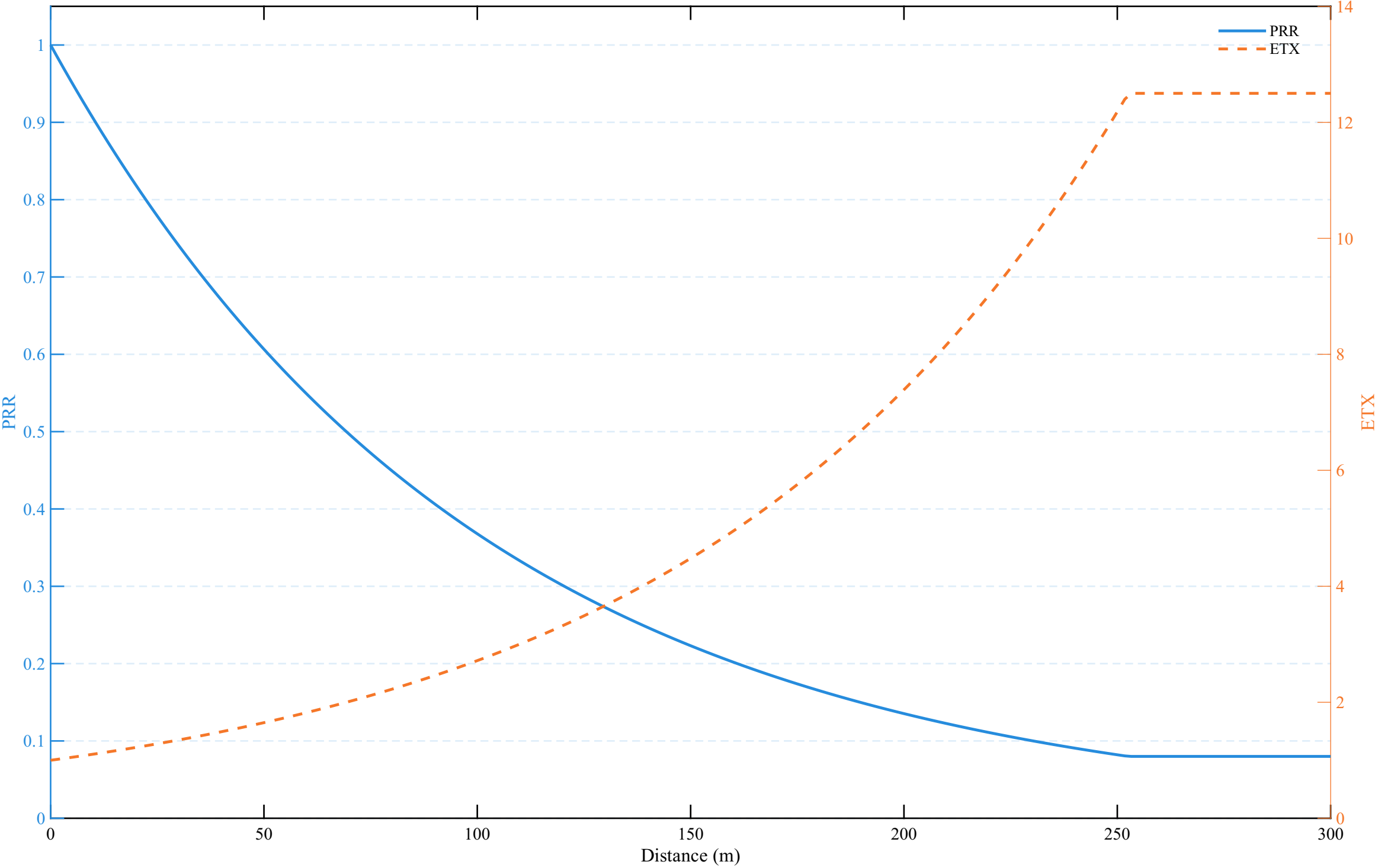
F1-3 PRR / ETX vs Distance
