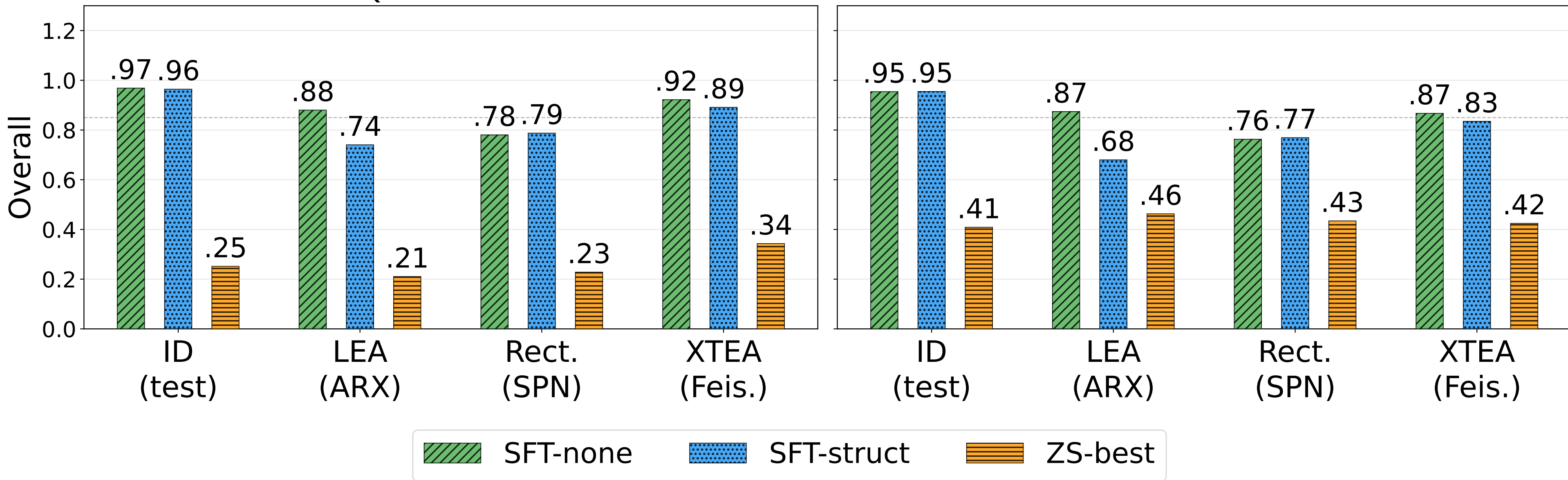
In-Distribution vs Unseen Cipher — Overall Score Qwen2.5-7B DS-Coder-V2-Lite
