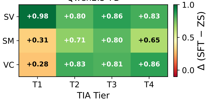
Qwen2.5-7B
