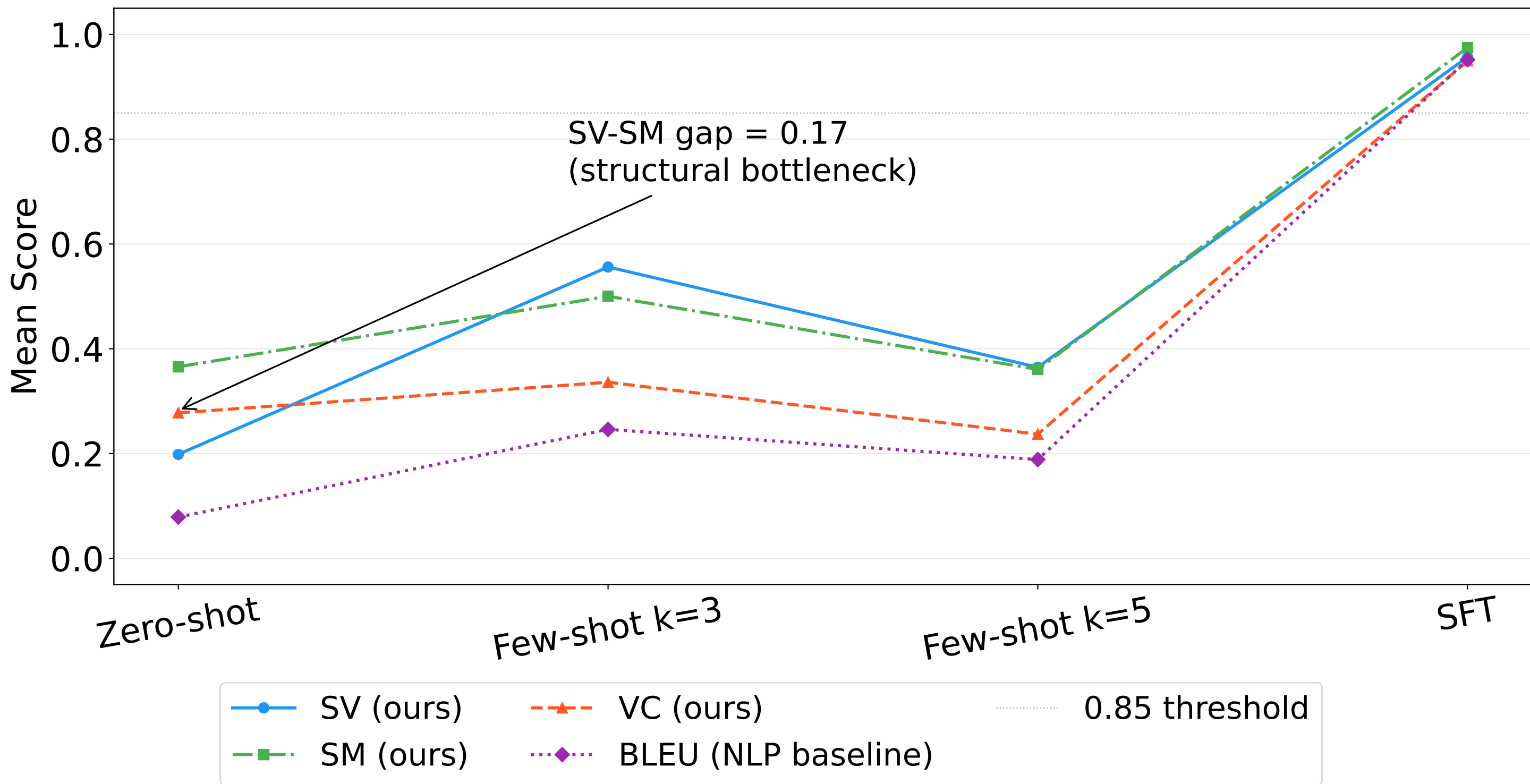
Mean Metric Values by Regime: SV/SM/VC vs BLEU (both models, test split)
