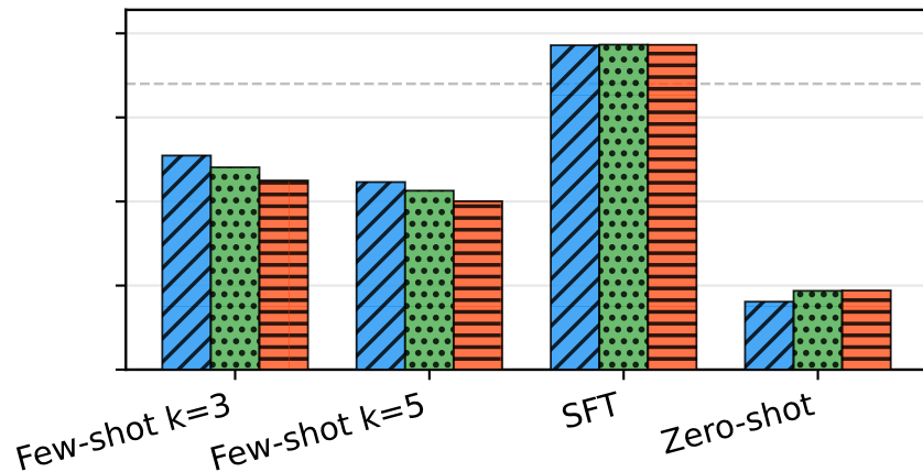
Qwen2.5-7B
