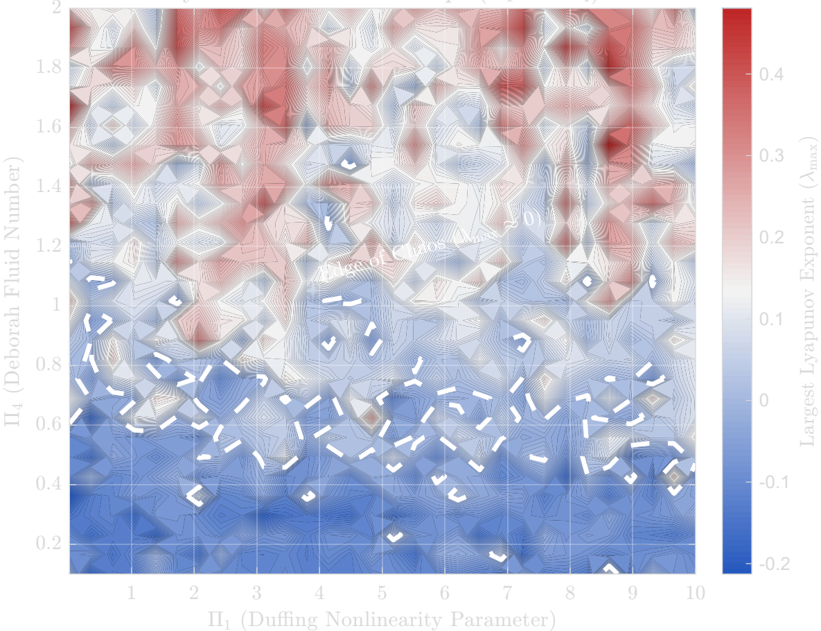
Dynamical Chaos Landscape ( \Pi_1 vs. \Pi_4 )
