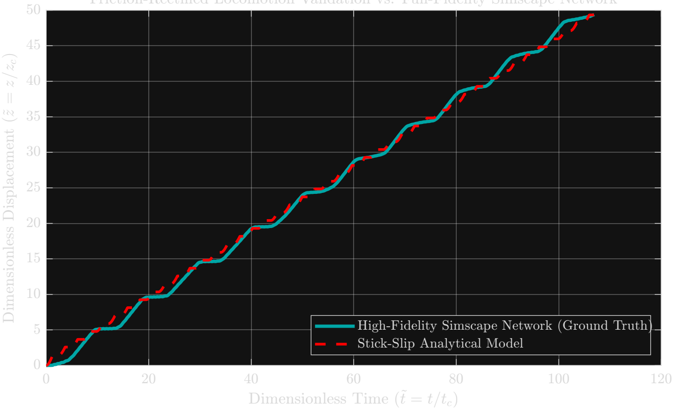
Friction-Rectified Locomotion Validation vs. Full-Fidelity Simscape Network
