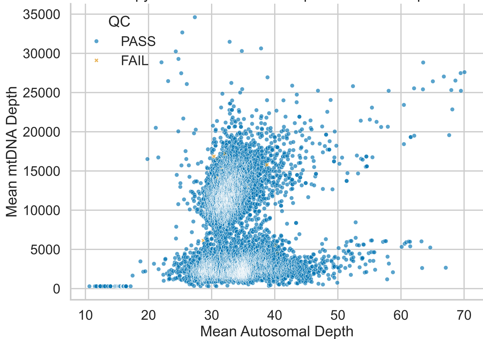
CopyNumber: Autosomal Depth vs mtDNA Depth
