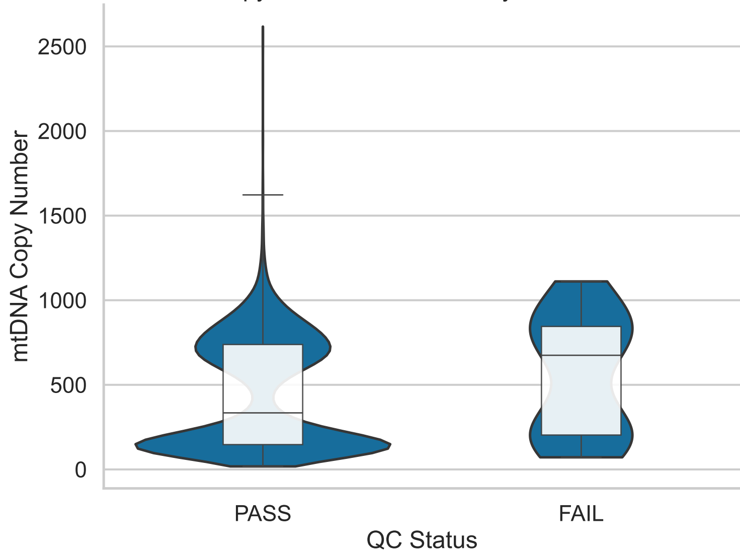
CopyNumber Distribution by QC Status
