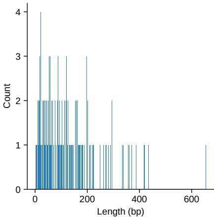
NUMT length distribution
