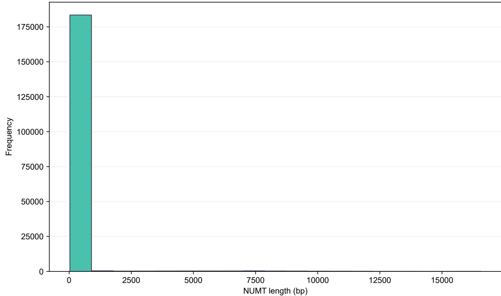
NUMT length distribution
