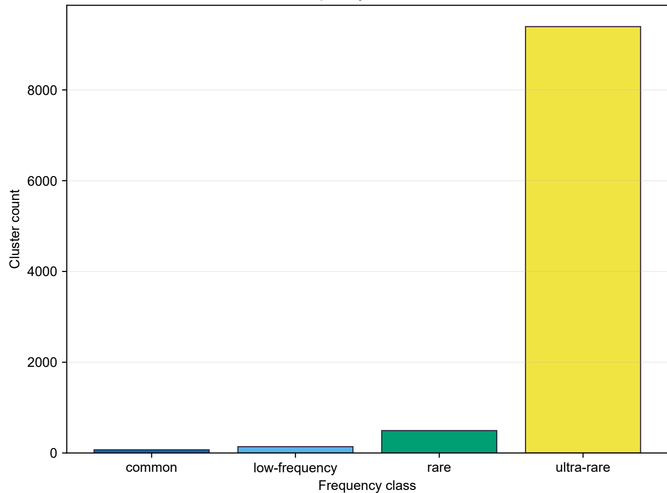
NUMT frequency class distribution
