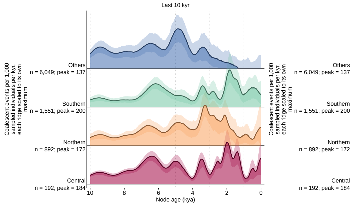
Coalescent event density by Corridor_NCS
