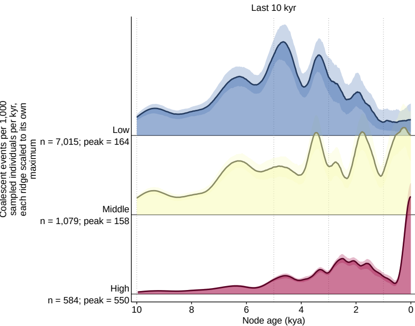
Coalescent event density by Elevation_group
