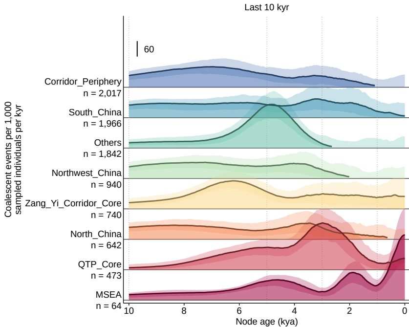
Coalescent event density by Corridor_and_key_regions
