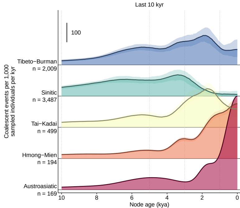
Coalescent event density by Language family
